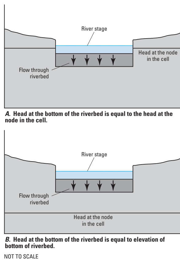
Figure 6-8. Diagram of cross sections showing the relation between head at the bottom of the riverbed layer and head in the cell. Head in the cell is equal to the water-table elevation. Figure modified from Harbaugh (2005).
