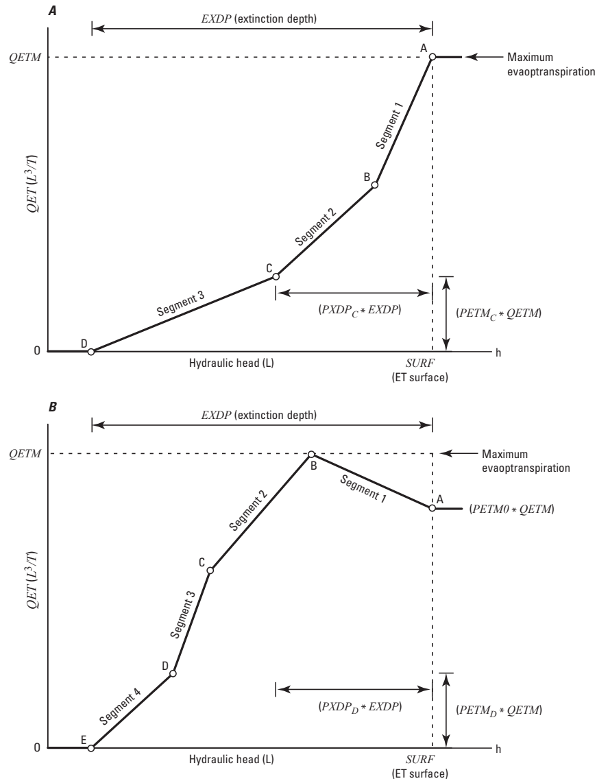
Figure 6–15. Graphs showing volumetric evapotranspiration (ET) rate, QET , as a function of head for two situations in which the function in the variable interval is defined using multiple segments. EXDP is the extinction depth, SURF is the ET surface, and QETM is the product of the maximum ET flux rate and the cell area. In A, the maximum ET rate applies at SURF , and PETM_C and PXDP_C define the location of point C. In B, the ET rate that applies at SURF is defined by the product of the optional variable PETM_0 and QETM .
