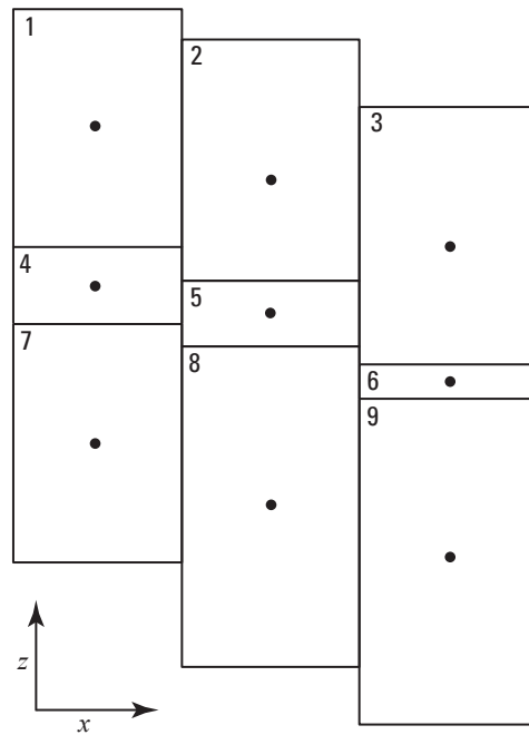
Figure 3-5. Diagram of cross section through a model grid used to demonstrate the concept of a horizontal connection and a vertically staggered horizontal connection. For a traditional MODFLOW representation in which a cell connects to only one other cell in a horizontal direction, the horizontal connection should be marked with an IHC value of 1 (for example, the intent is that cell 8 is connected on its right face only to cell 9). For a vertically staggered connection in which a cell may connect to more than one cell in a horizontal direction, the horizontal connection is vertically staggered and should be marked with an IHC value of 2 (for example, the intent is that cell 8 is connected on its right face to cells 3, 6, and 9). Vertically staggered horizontal connections can be specified for the unstructured Discretization (DISU) Package, but not for the structured Discretization (DIS) and Discretization by Vertices (DISV) Packages.
