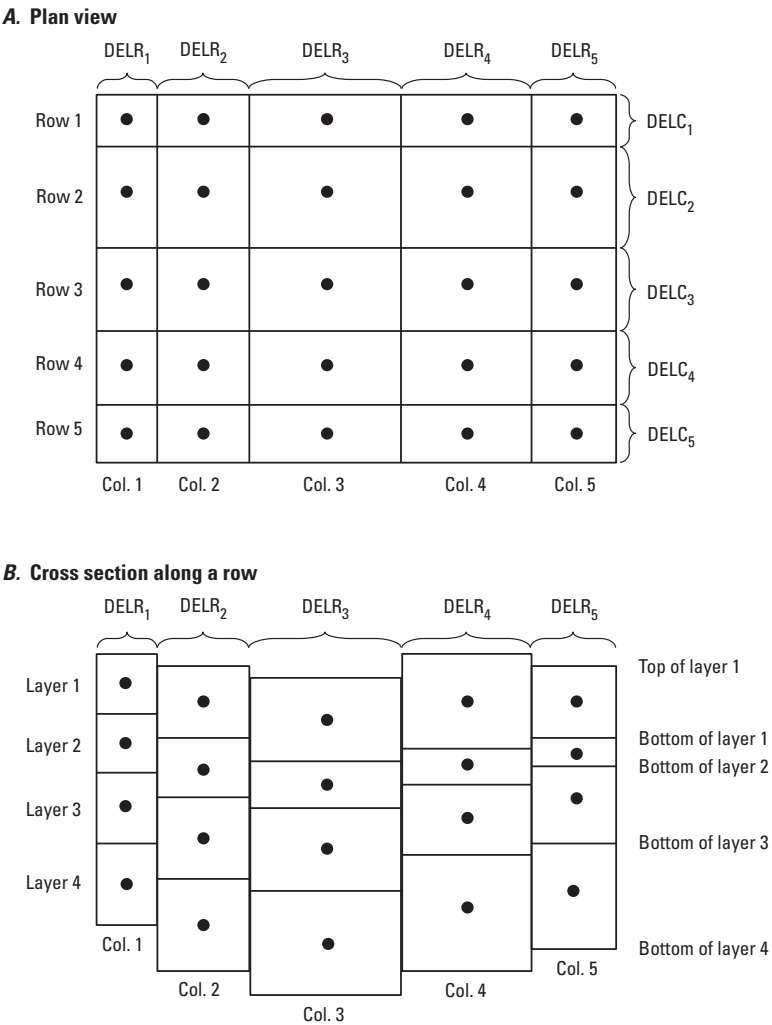
Figure 3–1. Diagram showing a regular MODFLOW grid. A , plan view, and B , cross-section view. Figure modified from Harbaugh (2005) .
