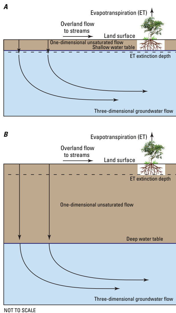
Figure 7-14. Diagram showing flow through the unsaturated zone. A , shallow water table, and B , deep water table. Figure modified from Niswonger and others (2006) .
