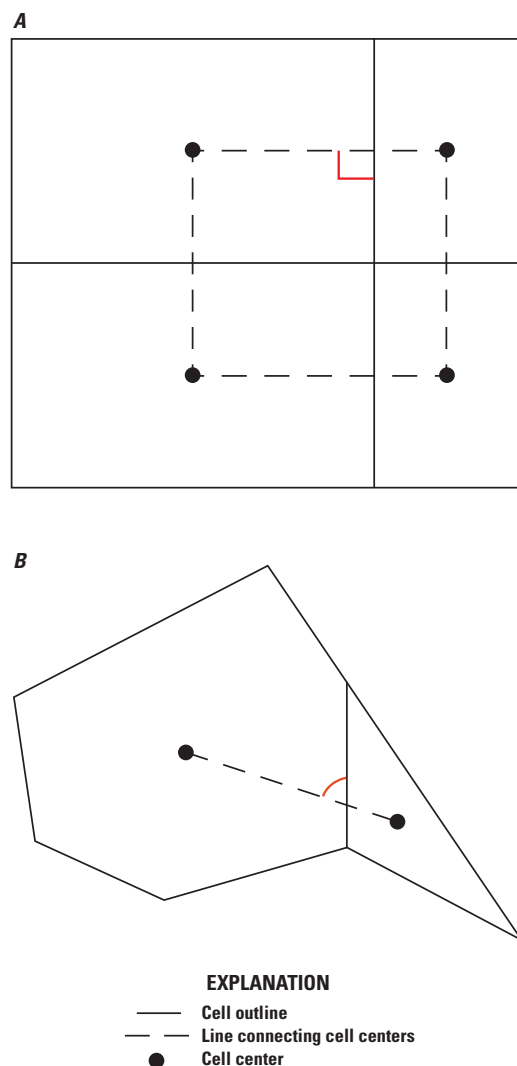
Figure 2-3. Diagram showing examples of two different types of cell connections. A , a line connecting the centers of adjacent cells passes through the shared face at a right angle; and B , a connecting line does not intersect the shared face at a right angle. Figure modified from Panday and others (2013).
