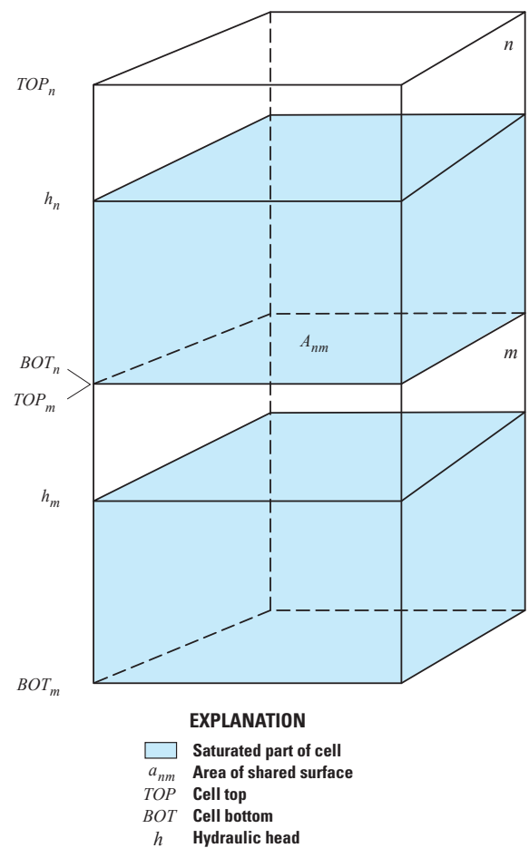
Figure 4-6. Diagram showing the situation in which a correction is required to limit the downward flow from cell n into m , as a result of cell m being partially dewatered. Figure modified from Panday and others (2013).
