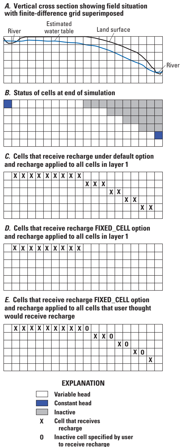
Figure 6-2. Diagram showing the cells receiving recharge under the default option, which is based on applying recharge to the highest active cell, and the cells receiving recharge under the FIXED_CELL option. These options are available in the Recharge Package. Figure modified from Harbaugh (2005) .
